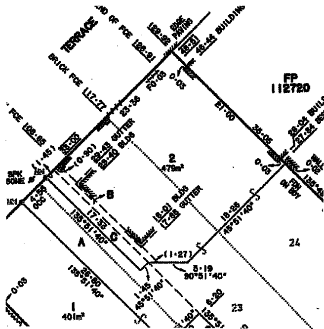
SITE PLAN (LOT 2)
